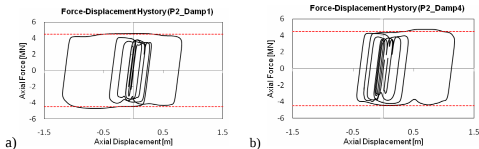
Figure 10. Nonlinear Viscous Damper hysteretic loops: a) Pier P2 - Horiz. Damper , b) Pier P2 – Verit. Damper
