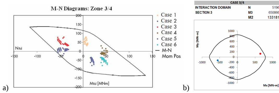
Figure 9. M-N interaction Diagrams: a) Composite deck – b) Tower 1/2 - \rho_{sl} = 3.5\% , A_{sl,tot} = 9765 \text{ cm}^2
