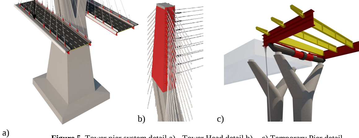
Figure 5. Tower pier system detail a) - Tower Head detail b) - c) Temporary Pier detail
