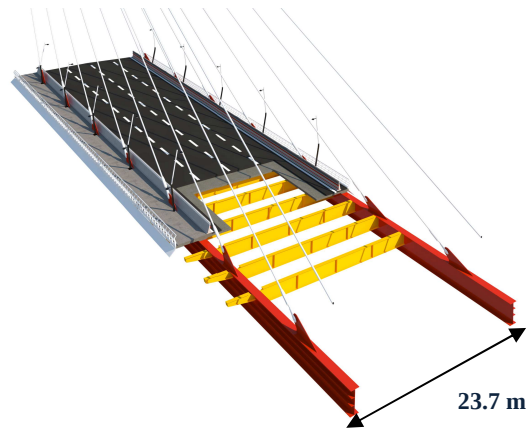
Figure 3. Bridge deck detail
