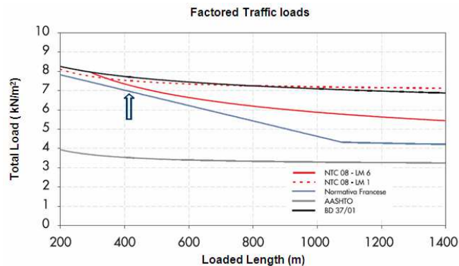
Figure 6. Traffic load comparison for loaded lengths greater than 200 m.
