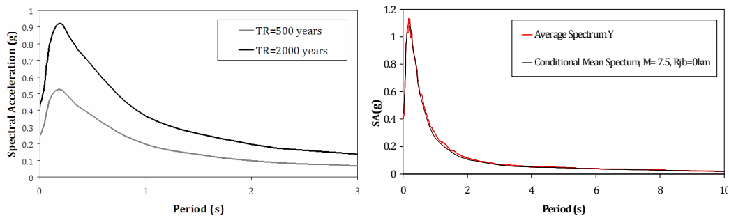
Figure 8. UHS for 500 and 2000 years Return Periods a) - Target Spectrum match ( Y - transv. direction).
