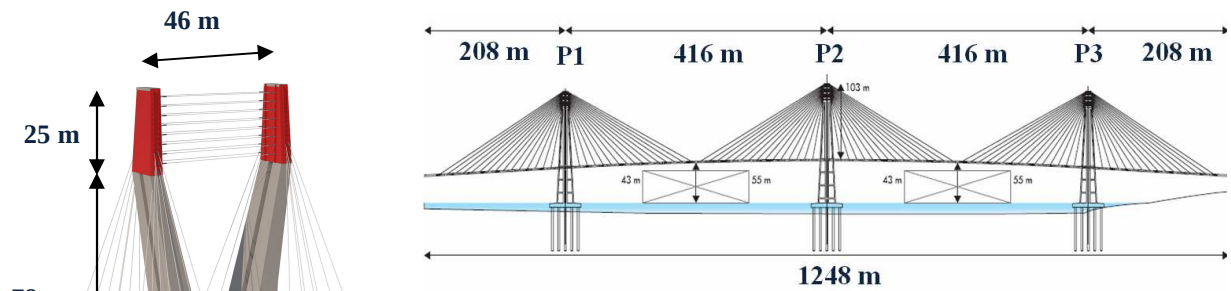
Figure 4. SCB Longitudinal Profile
